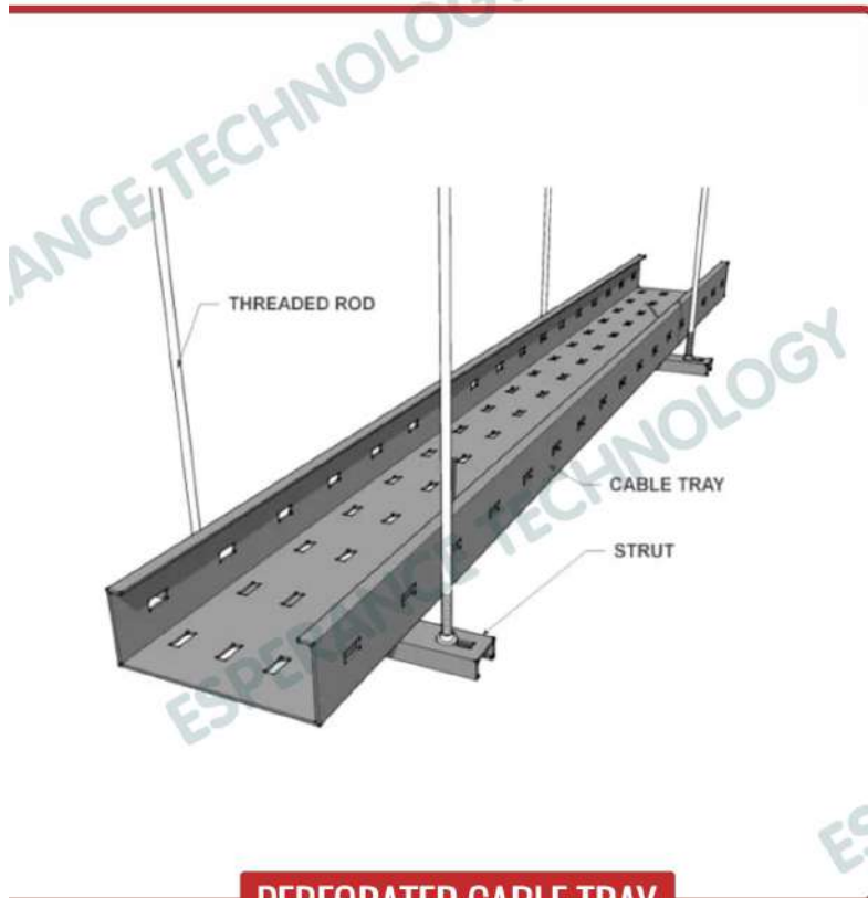
PERFORATED CABLE TRAY
